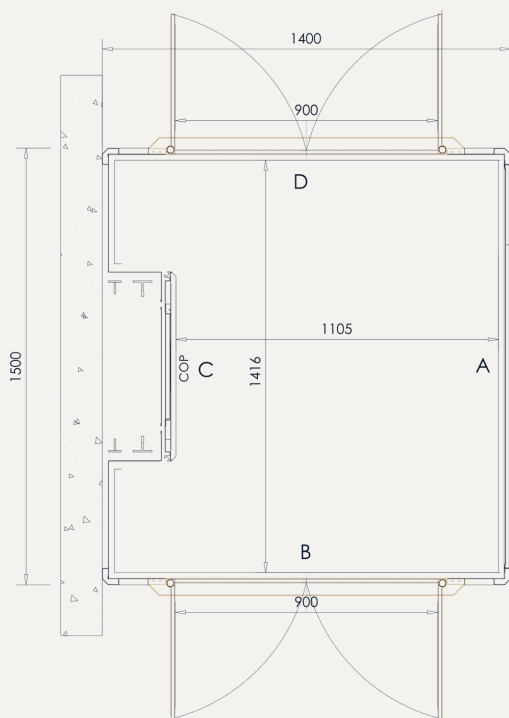
Plan: 1,100 x 1,400mm platform with through entry, in a 1,400 x 1,500mm shaft (400kg).
