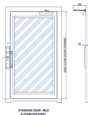
Standard door Mild and stainless steel
