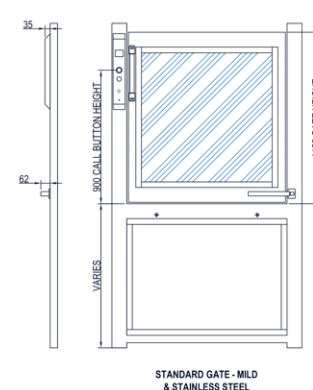
Standard gate Mild and stainless steel
