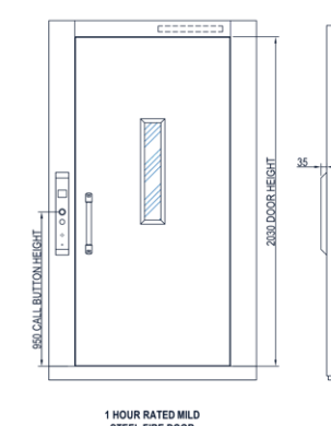
One-hour fire door Mild steel
