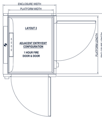
Layout 2 Adjacent entry
