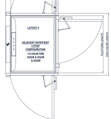
Layout 4 Adjacent entry, 3 stop
