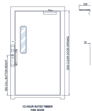
Half-hour fire door Timber
