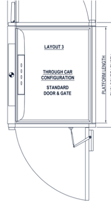
Layout 3 Through car
