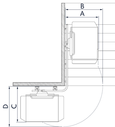
RAIL WITH 90°-CURVE
